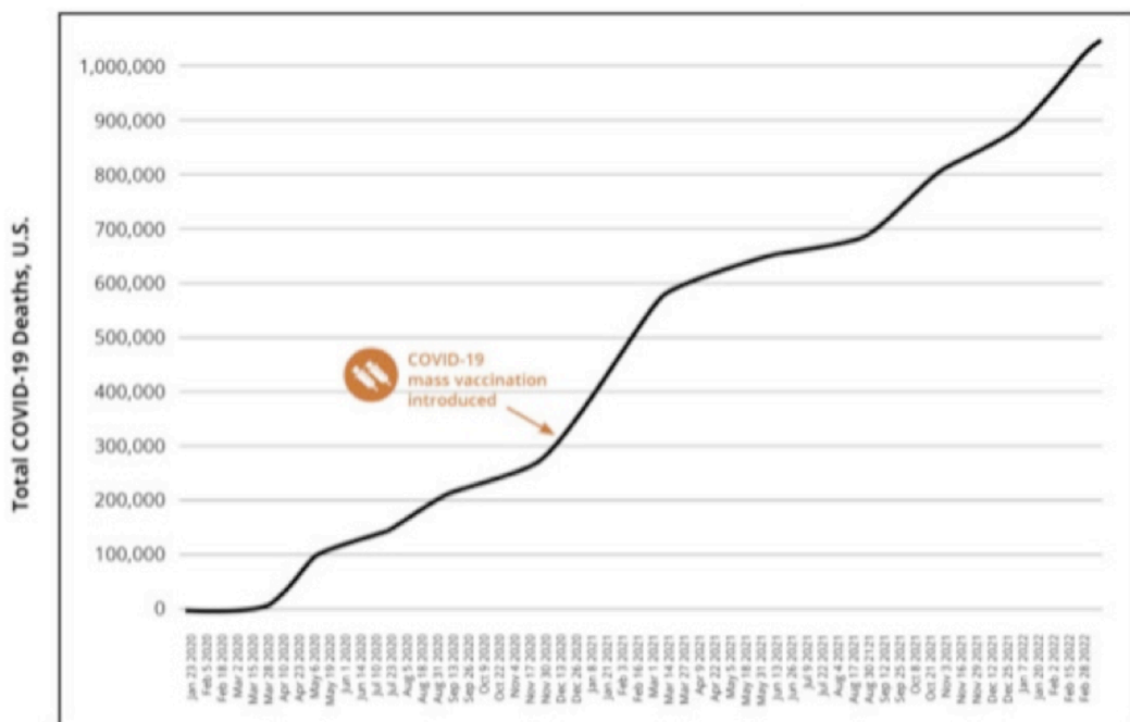
COVID-19 Pre-Vaccine vs. Post-Vaccine Mortality Rate, United States
